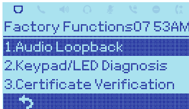
Factory Functions
