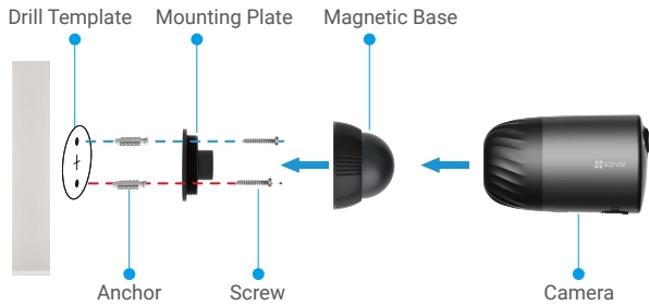
Fig. 2 Secure by magnetic base
